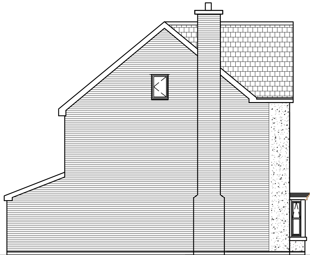
SIDE ELEVATIONS
